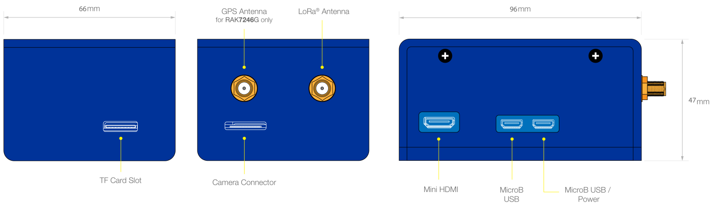
Figure 2: Hardware Interfaces
