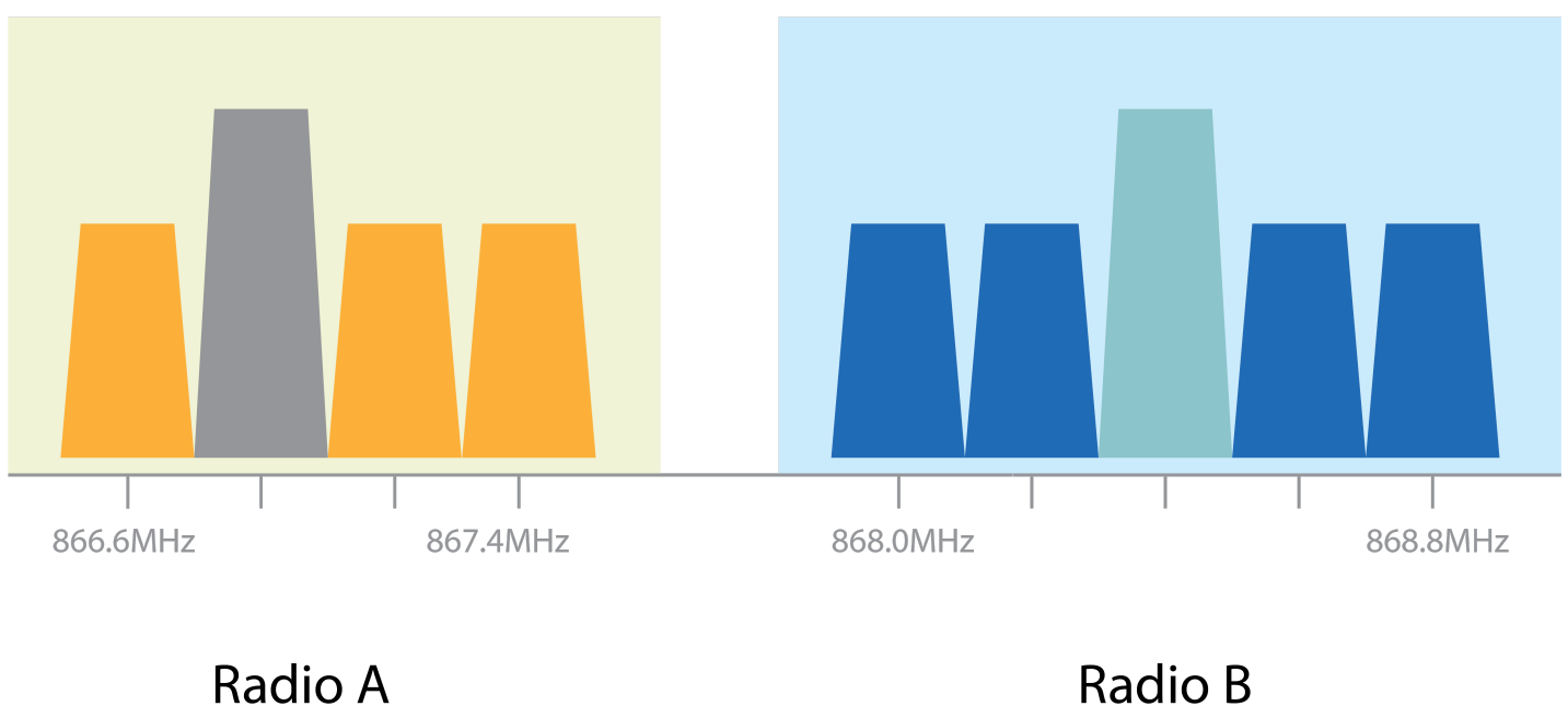
Figure 6: LoRa Channel
