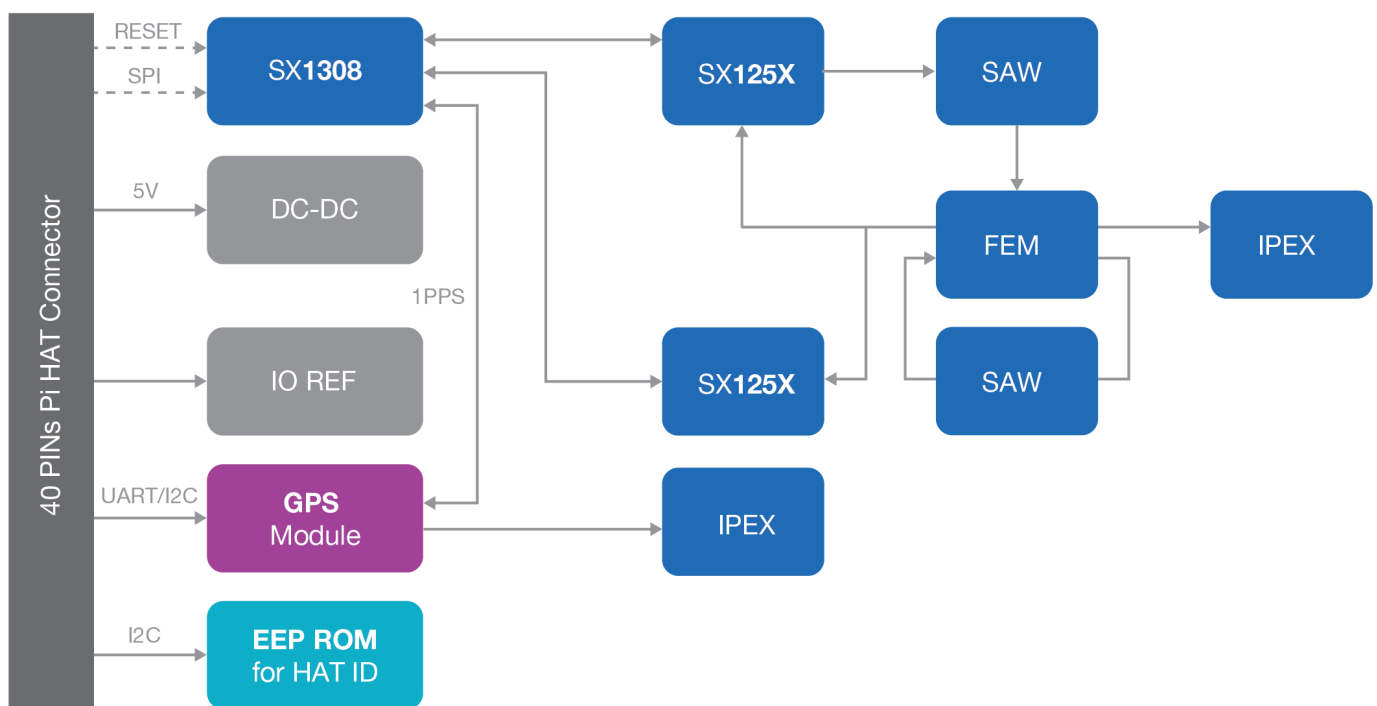
Figure 5: Block Diagram
