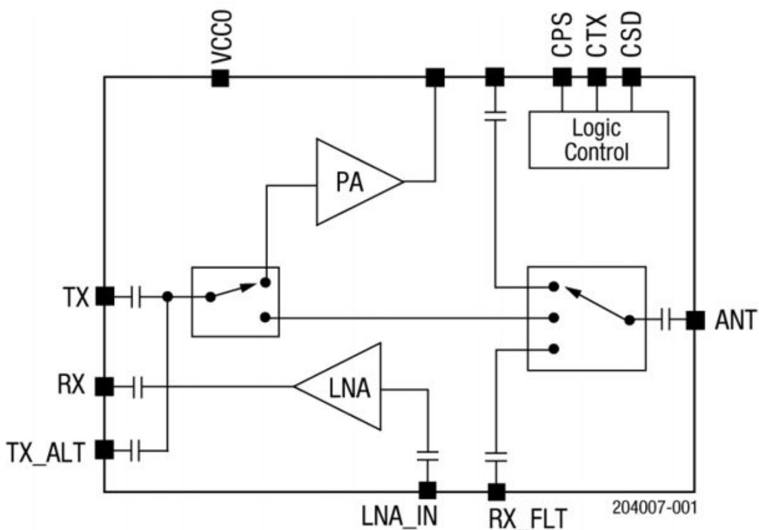
SKY66422-11 Block Diagram
