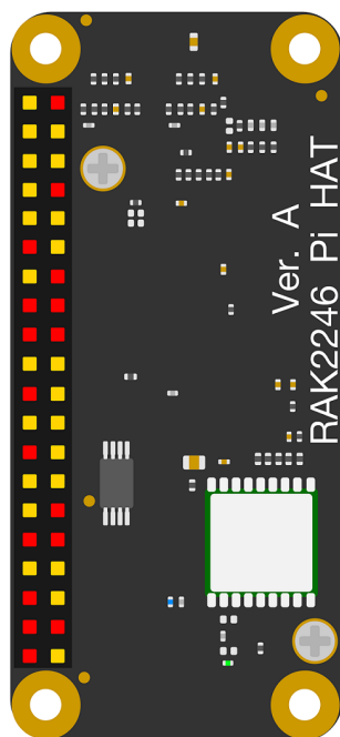
BOTTOM VIEW
