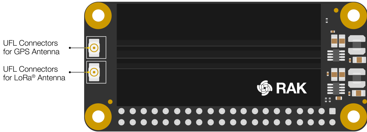
Figure 1: uFL Connectors for LoRa and GPS
