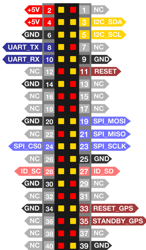
Figure 7: RAK7246G Pinout Diagram
